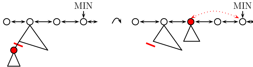
Abbildung 2.55: Skizze: Operation decrease_key
